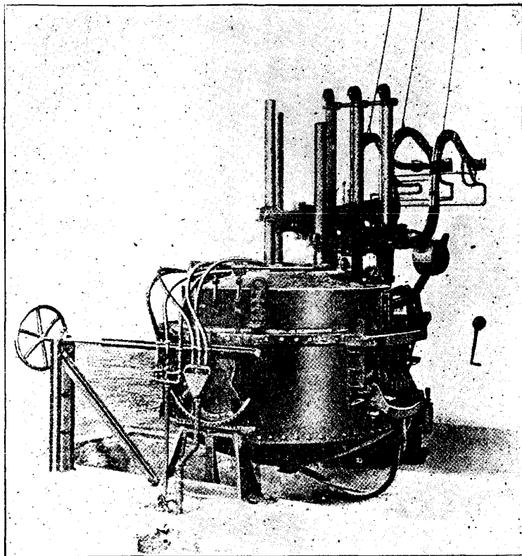
This furnace is using 3-inch Acheson Electrodes melting cold scrap on a basic bottom for alloy steel castings. It is a 1/2-ton Moore Rapid' Electromelt Steel Furnace.
