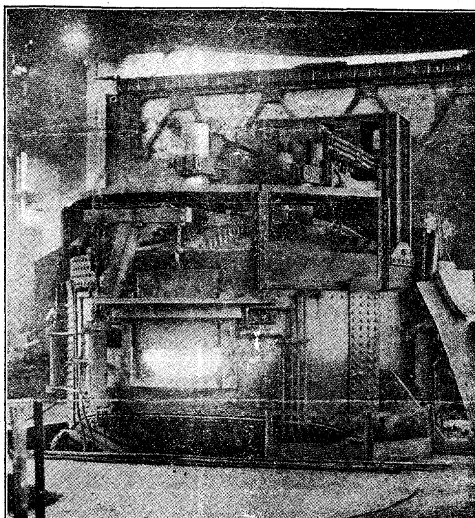
This furnace is using 12-inch Acheson Electrodes refining hot metal in a duplex process on a basic bottom, making special steel for ingots. It is a 25-ton Heroult Furnace.
