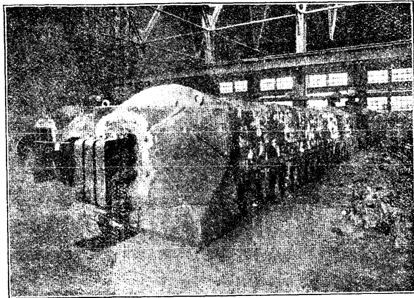
FURNACE IN WHICH ACHESON-GRAPHITE IS MADE
