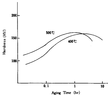
Fig. 1 Effect of aging time and temperature on hardness.
