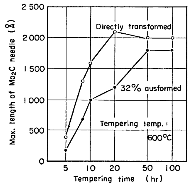
Fig. 5. Growth of Mo 2 C needle crystal during isothermal tempering at 600°C, showing difference between ausformed and directly transformed specimens (alloy M1).
