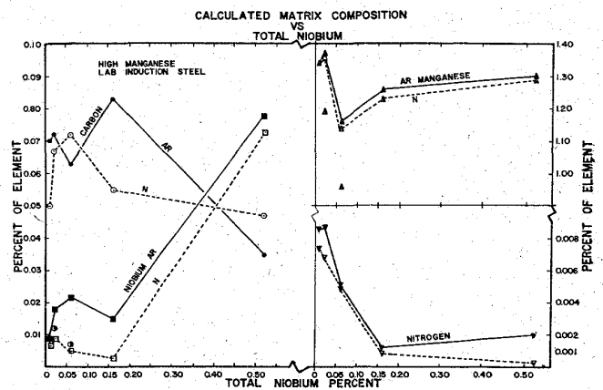
Fig. 14. Calculated matrix composition. High manganese group of steels.
