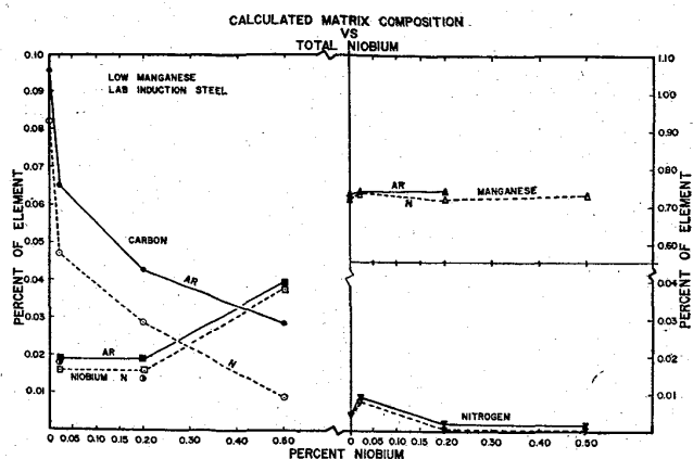
Fig. 16. Calculated matrix composition. Low manganese group.
