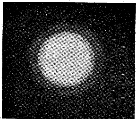
Photo. 5. Electron diffraction pattern of 0.023% niobium steel.
