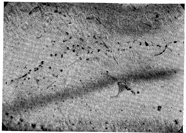
Photo. 4. Electron micrograph of normalized 0.023% niobium steel. Electron transmission,
