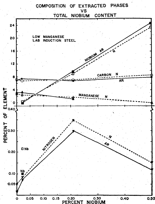
Fig. 15. Chemical composition of the extracted phases. Low manganese group.
