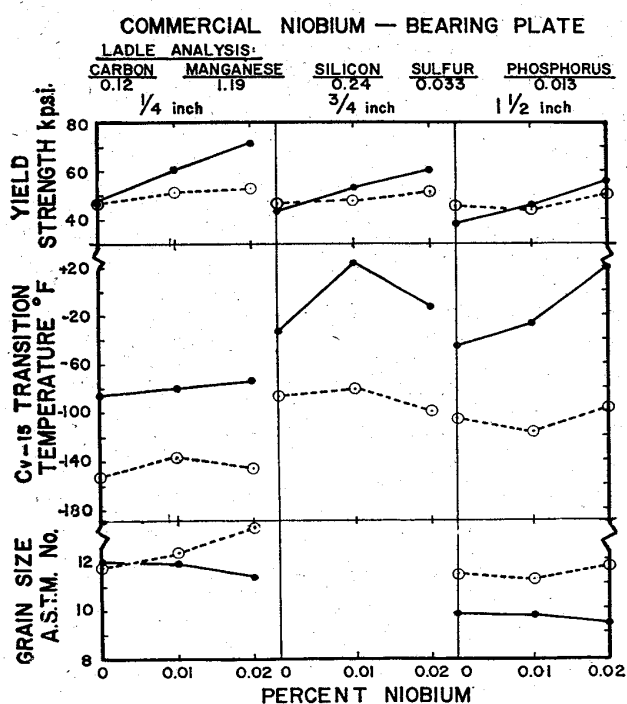
Fig. 9. The influence of niobium on the yield strength, the transition temperature and the grain size of commercial niobium-bearing plate.
