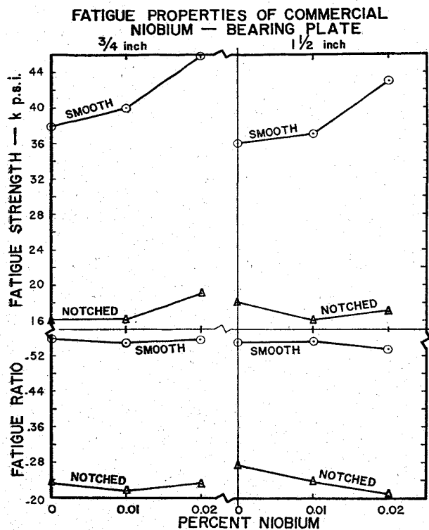
Fig. 10. The influence of niobium on the fatigue characteristics of commercially-produced niobium-bearing steel.
