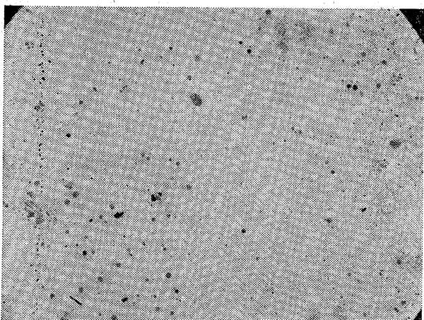
Photo. 3. Electron micrograph of normalized 0.07% niobium steel. Carbon extraction replica.
