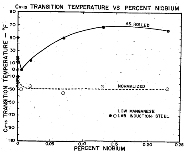
Fig. 7. The influence of niobium on the Charpy V-notch 15ft-lb transition temperature of low manganese steels.
