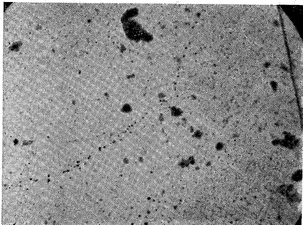
Photo. 2. Electron micrograph of normalized 0.23% niobium steel. Carbon extraction replica.
